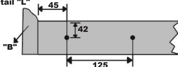
Detail "L"
