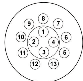
Contact description in 13-pin socket
